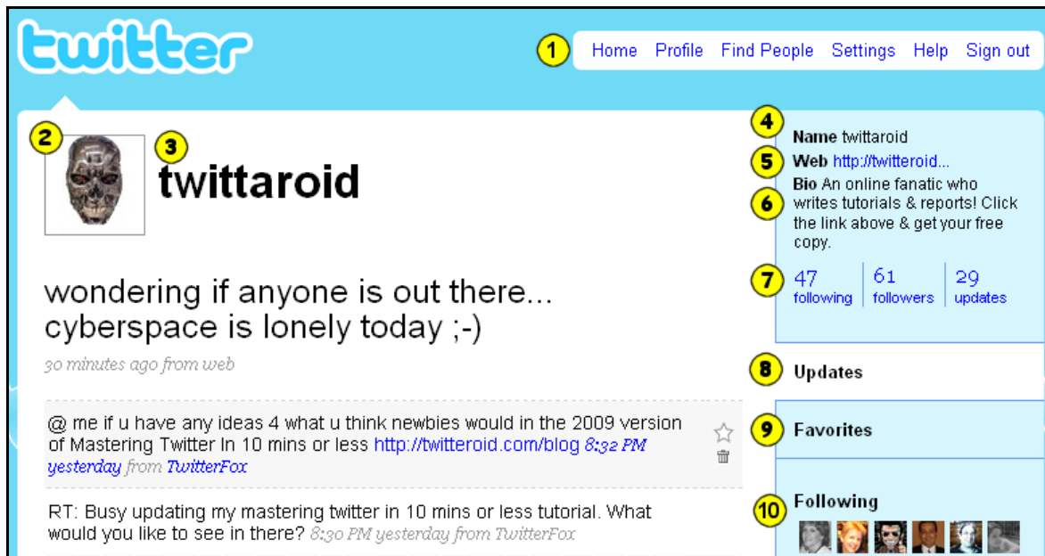
Figure 3-3: Twitter Explained
